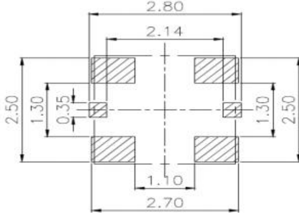
推荐钢网/RECOMMEND METAL MASK (钢网厚度/Mask thickness 0.12mm)
